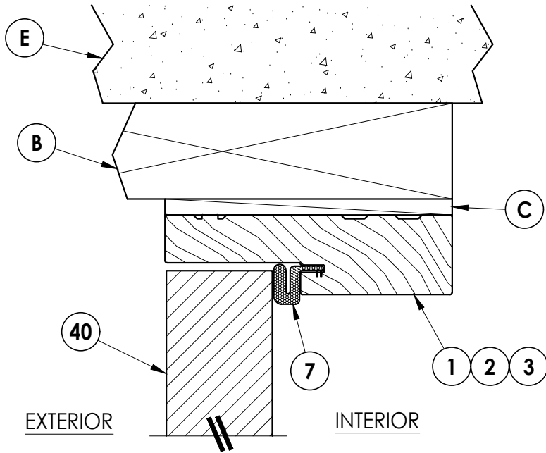
1 4 VERTICAL CROSS SECTION Outswing shown (Inswing similar) Shown w/ 2X Buck
