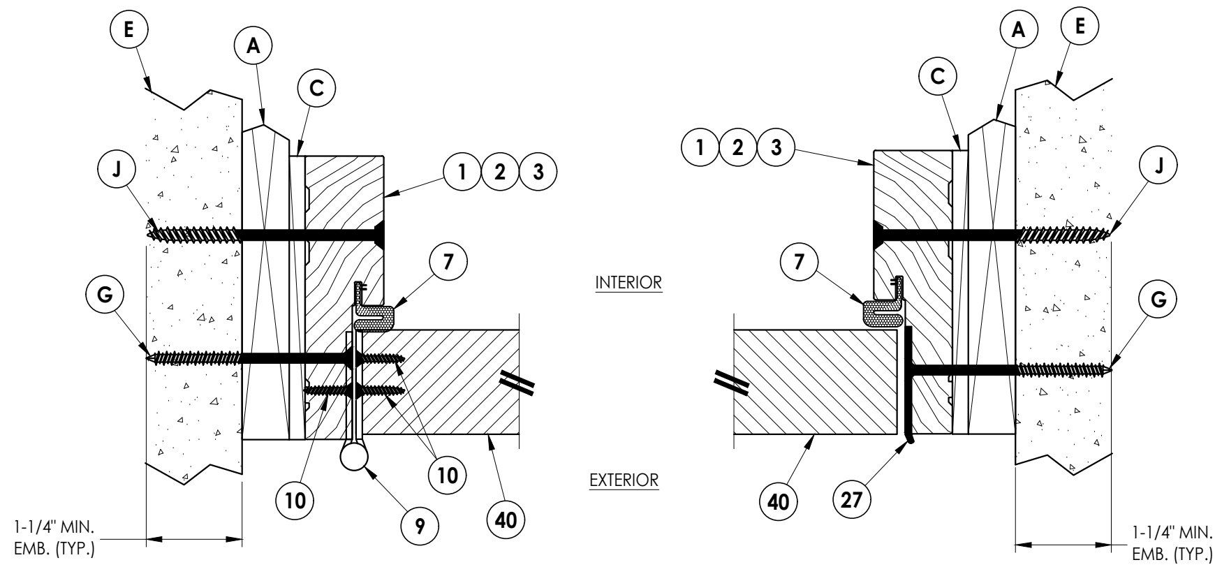
2 HORIZONTAL CROSS SECTION 5 Outswing shown (Inswing similar) Shown w/ 1X Buck
