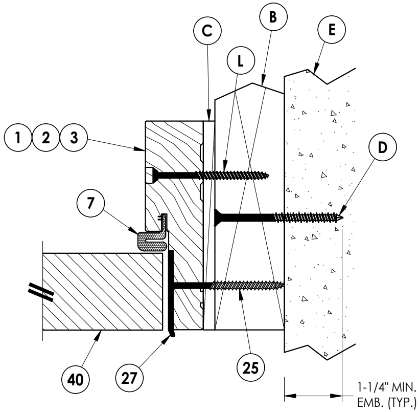
1 4 VERTICAL CROSS SECTION Outswing shown (Inswing similar) Shown w/ 2X Buck
