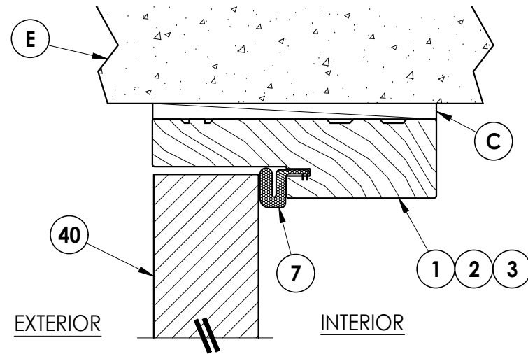
1 6 VERTICAL CROSS SECTION Outswing shown (Inswing similar) Shown Direct to Masonry
