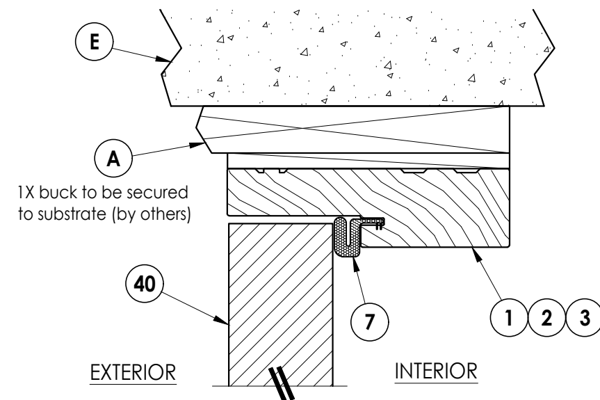
1 VERTICAL CROSS SECTION 5 Outswing shown (Inswing similar) Shown w/ 1X Buck
