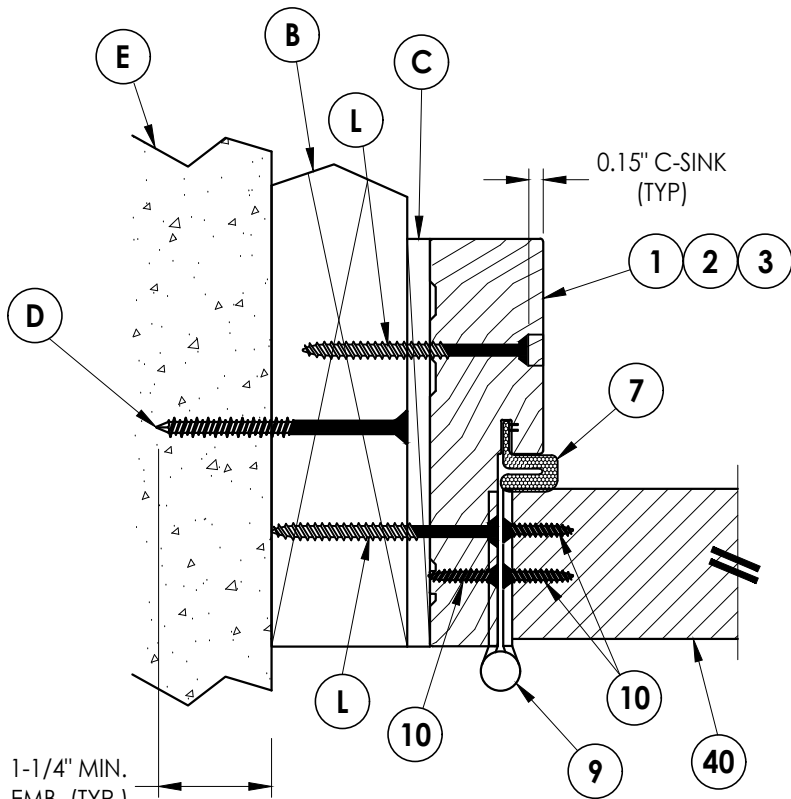
2 4 HORIZONTAL CROSS SECTION Outswing shown (Inswing similar) Shown w/ 2X Buck
