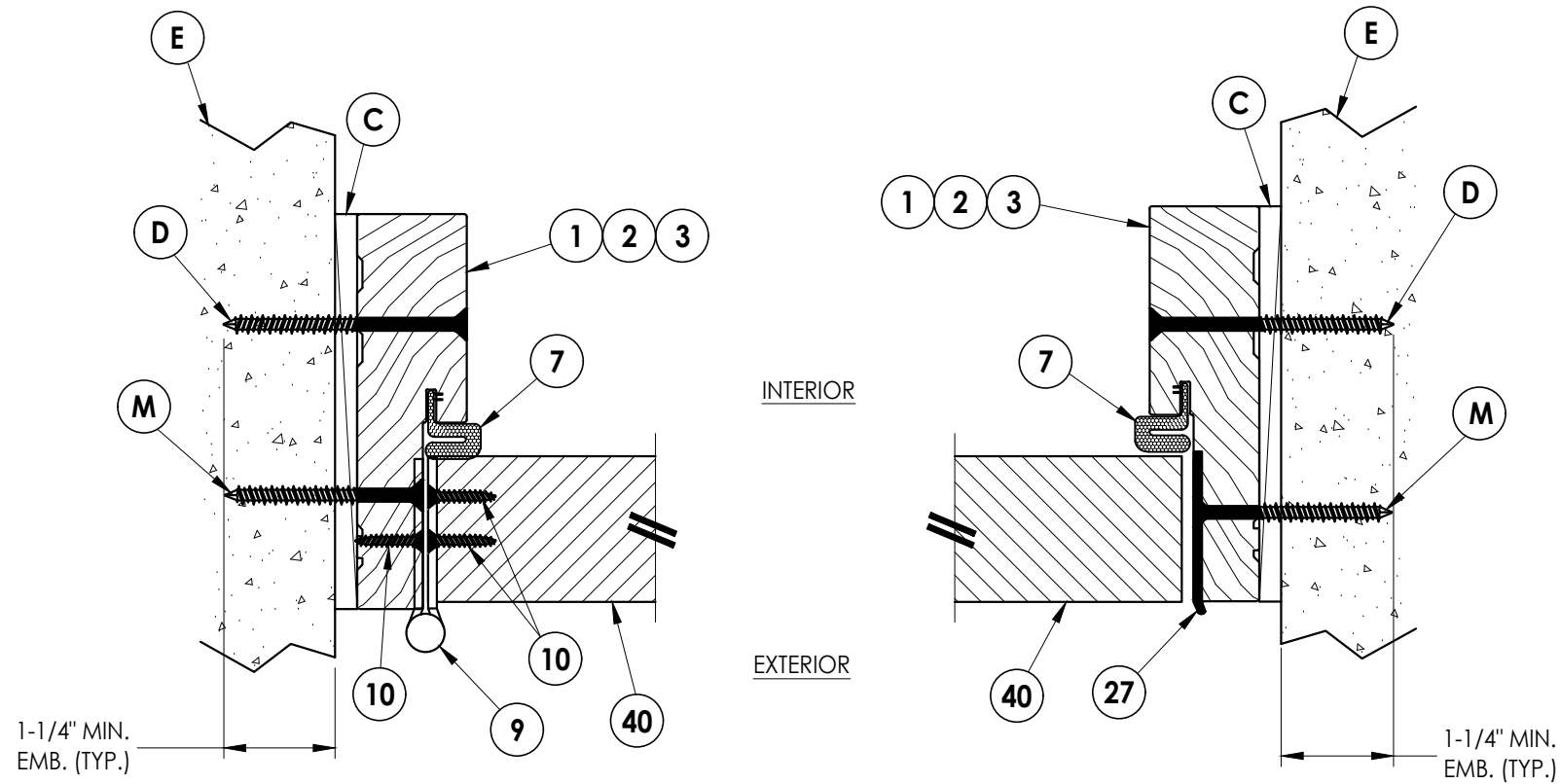
2 HORIZONTAL CROSS SECTION 6 Outswing shown (Inswing similar) Shown Direct to Masonry
